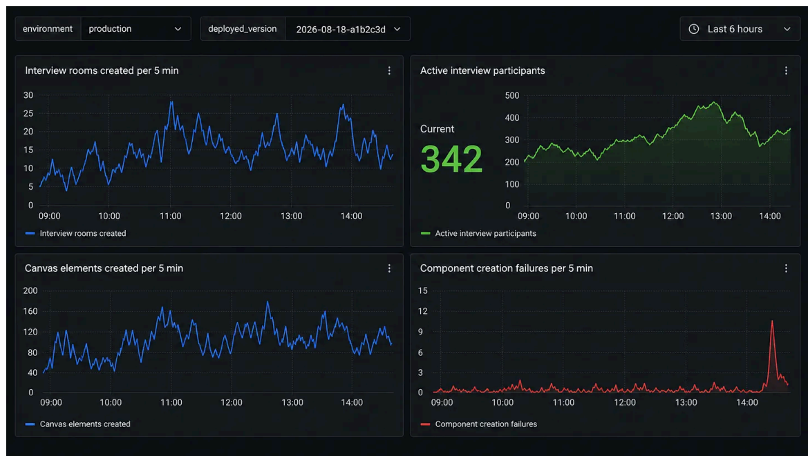
Grafana dashboard with the metrics
